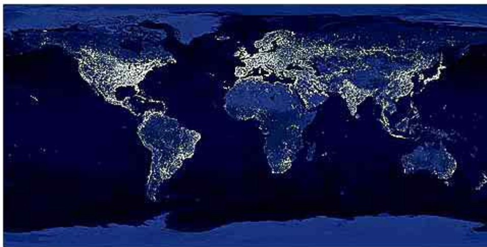
The World at Night (from Satellite Imaging)
